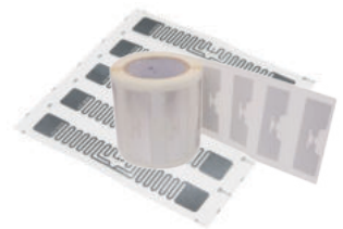
AGS-U-TG30 UHF Windshield Tags Non Tearable 860-960 MHz
