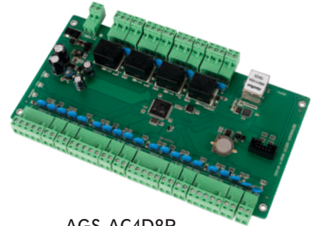
AGS-AC4D8R 4 Door / 8 Reader Communication : LAN Register Cards : 42000 Record Capacity : 200000 Camera can be Integrate Input: Wiegand26/34
