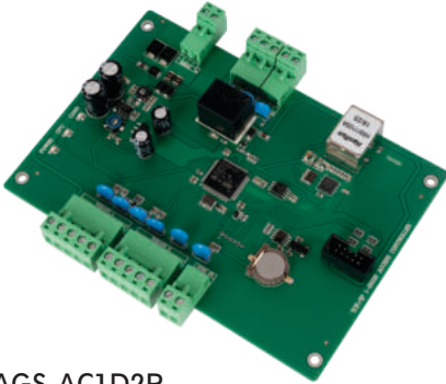
AGS-AC1D2R 1 Door / 2 Reader Communication : LAN Register Cards : 42000 Record Capacity : 200000 Camera can be Integrate Input: Wiegand26/34
